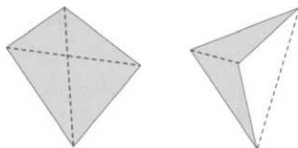
FIGURE 11.7. A convex and a concave quadrilateral.
