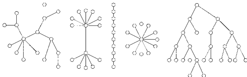
FIGURE 8.1. Five trees.
