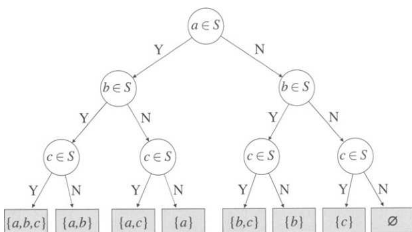
FIGURE 1.2. A decision tree for selecting a subset of \{a, b, c\} .
