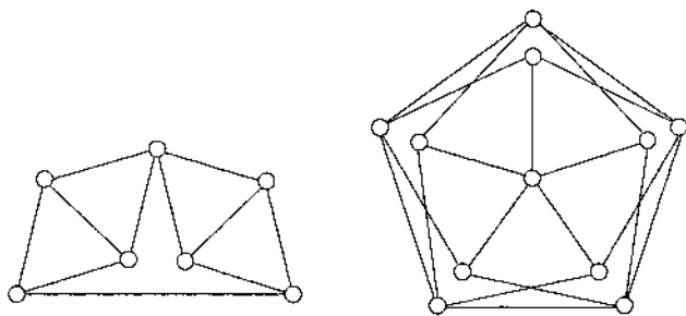
FIGURE 13.6. Two non-3-colorable graphs.
